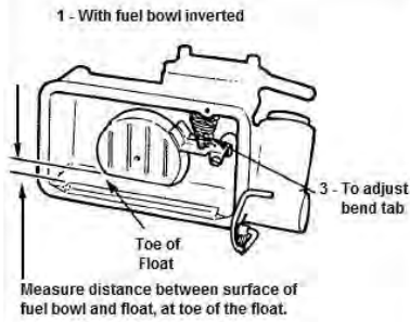
FIG. 4 - DRY FLOAT SETTING
