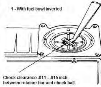
FIG. 5 - PUMP INTAKE CHECK BALL ADJ.
