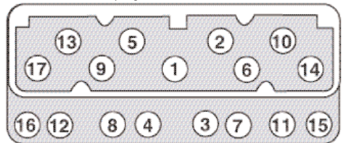
Figure 2 - Cylinder Head Bolt Torque Sequence Torque Bolts to 65 ft./lbs. in Three Steps (40-55-65)
